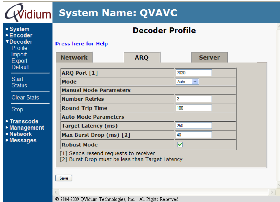
Figure 3b: Decoder profile: "ARQ Tab"
